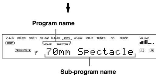
Sub-program name
